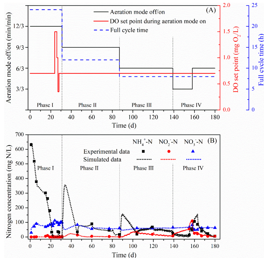
Figure 4. (A) The SBR operation strategies in different phases of the long-term experiment and (B) the experimental data and model simulated result of the SBR effluent in different phases.
