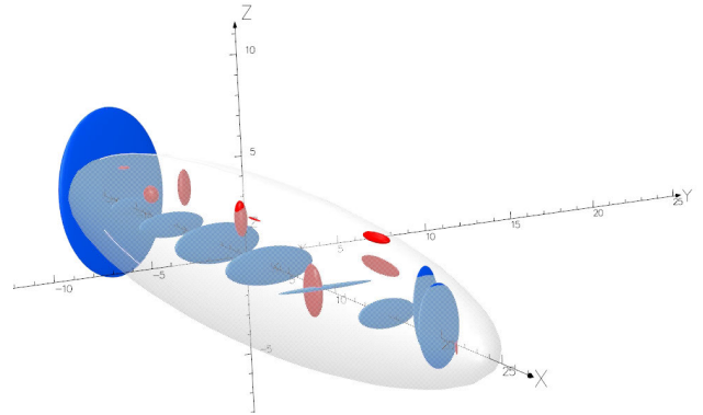
FIGURE 22. Visualization of dipole locations and relative values of magnetic moments in XYZ perspective (red – permanent dipoles, blue – induced dipoles).
