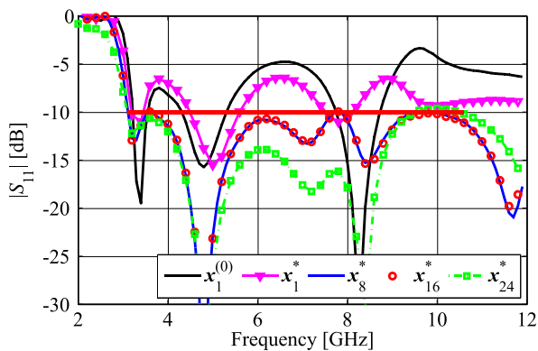
FIGURE 4. Comparison of the spline-parameterized antenna characteristics at the initial design (black) and the optimized designs obtained in each meta-iteration. Red horizontal line denotes the desired level of in-band matching.
