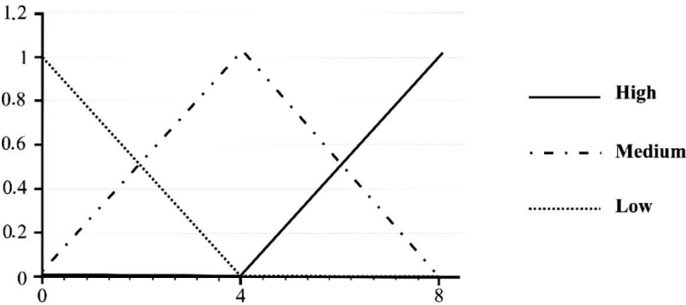
Figure 3. Fuzzification
