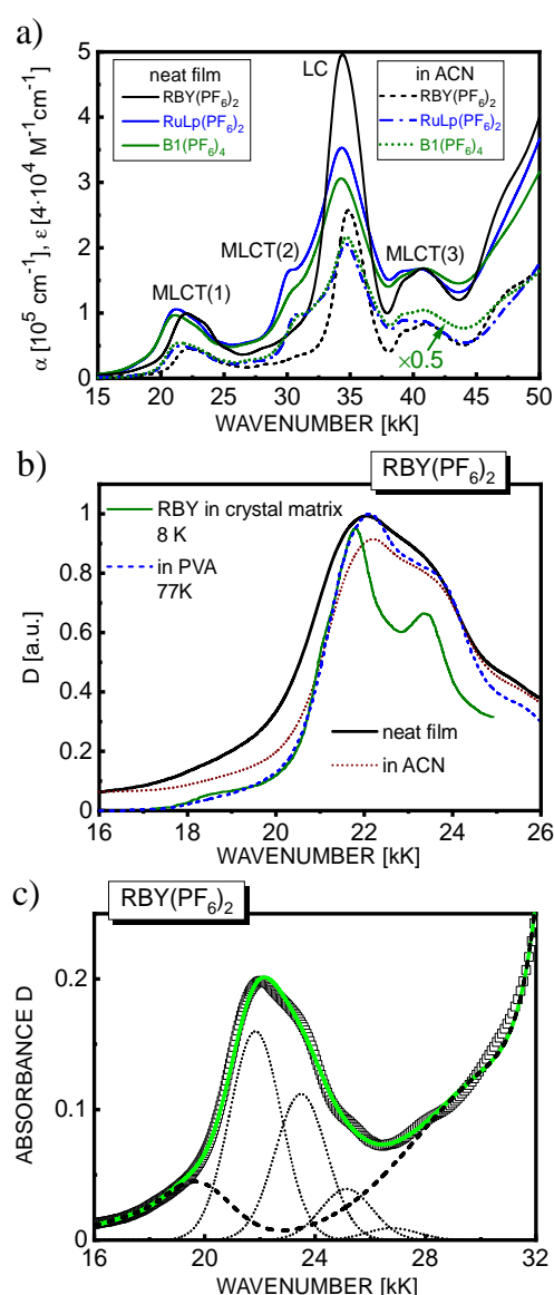
Figure 2. (a) Absorption spectra of RBY(PF 6 ) 2 , RuLp(PF 6 ) 2 , and B1(PF 6 ) 4 in neat films (solid lines) and in ACN solution (broken lines)—for colors, see the website. The molar extinction coefficient ( \epsilon ) of B1(PF 6 ) 4 was multiplied by 0.5. The spectral ranges of the MLCT and LC excited states are also indicated; (b) Comparison of absorption spectra in the MLCT(1) range for RBY(PF 6 ) 2 : in a neat film (thick solid line), in an ACN solution (dotted line), in a PVA matrix at 77 K (dashed line, data taken from [30]), and for RBY in the crystal matrix Zn(bpy) 3 (BF 4 ) 2 at 8 K (thin solid line, data from [12]); (c) Absorption spectrum of a 46 nm-thick RBY(PF 6 ) 2 film (squares) with the total fit (solid line) and its Franck–Condon components (dotted lines) in the MLCT(1) range ( \nu_0 = 21.84 kK, \Delta\nu = 1.65 kK, w = 2.2 kK and S = 0.7 ). The background from the lower energy and higher energy states is represented by a dashed line.
