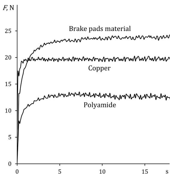
Fig. 6. Change in the friction force F in the regime of velocity step.
