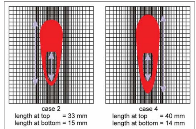
Fig. 15. Comparison of weld pool length at top and bottom of the plate due to the different thermal conductivity applied (in quasi-steady state) [31]
