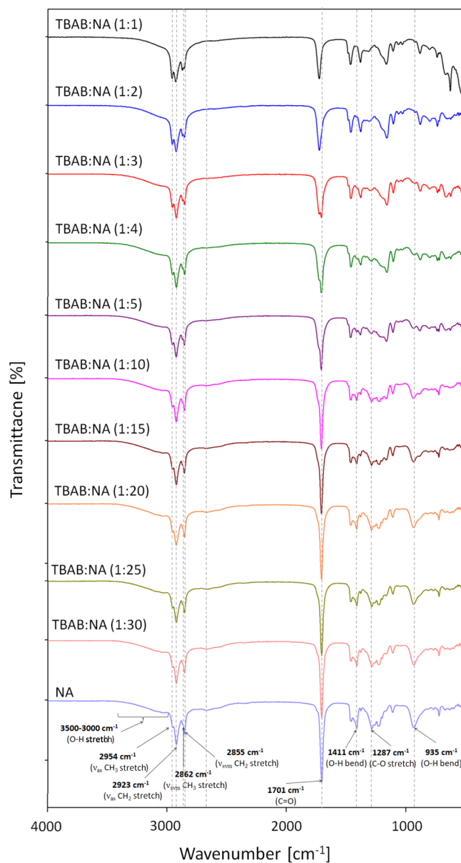
Figure 3. FT-IR spectra of DESs composed of TBAB and NA in various molar ratios and pure NA.
