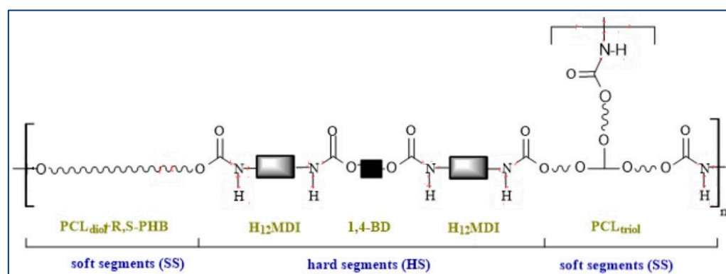
Scheme 2. Schematic representation of the chemical structure of polyesterurethanes.
