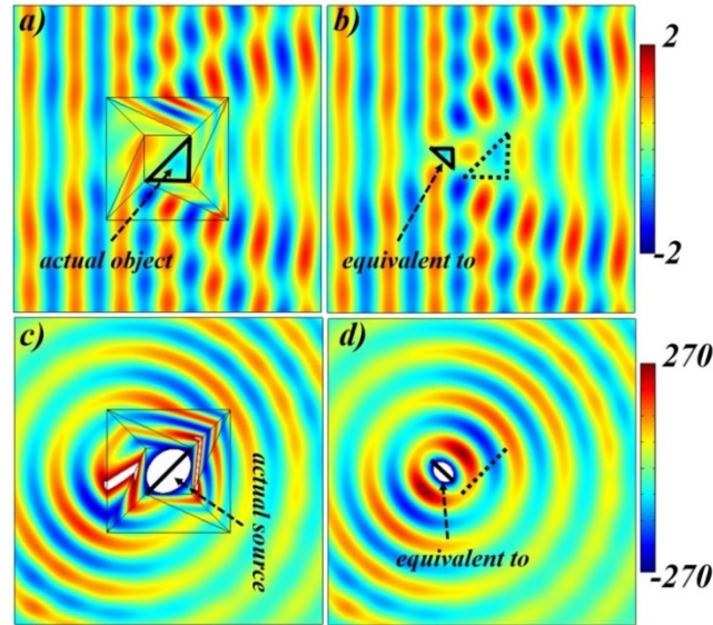
Fig. 5. Simulation results of both passive and active scatterer under shrinking-resaping device to achieve shrinking, reshaping and location shifting. (a) The z-directed electric-field's scattering behavior of big-sized dielectric object of \varepsilon = 5 and is \mu = 1 is placed in the core region of the proposed device that is optically equivalent to a smaller-sized object in a different position and location, as shown in (b). (c) E_z distributions of a big-sized line source with electric-field intensity of 1V under the proposed device is manipulated to achieve shrinking and location shifting. This gives the impression of the smaller-sized source's existence in a different position and location (d).
