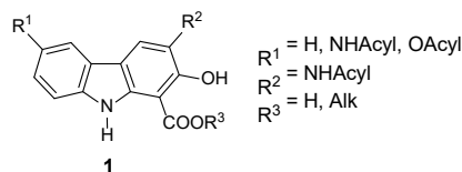
Figure 1. Structures of the newly designed carbazoles.
