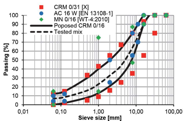
Figure 2 Proposed grading curves limits for CRM 0/16
