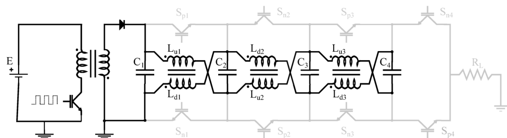
Figure 4. Charging phase.
