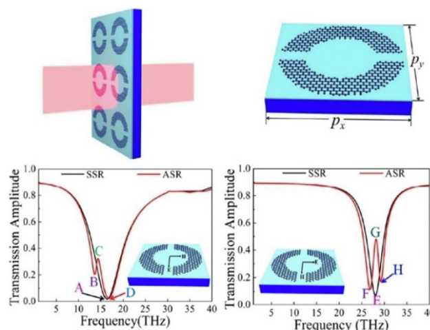
Fig. 4. The unit cell of the structure and simulated transmission amplitude curve (.), reproduced with permission from [169]
