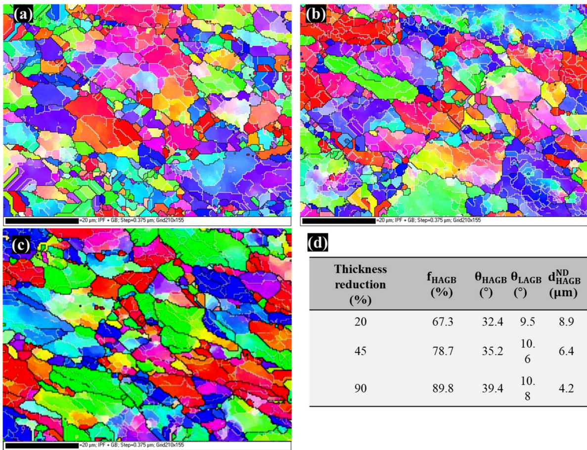
Figure 2. IPF maps of the Al/1 wt% CNT composites after (a) 20%, (b) 45%, and (c) 90% of thickness reduction, (d) HAGBs (high angle grain boundary-s) fraction ( f_{HAGB} ), LAGB (low angle grain boundary) and HAGB average misorientation angle ( \theta_{LAGB} , \theta_{HAGB} ) and HAGB spacing in normal direction ( d_{HAGB}^{ND} ) in rolled Al/1 wt% CNT composites.
