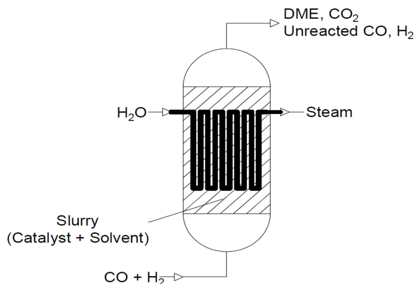
Figure 12. Scheme of a slurry reactor. Developed based on [1].
