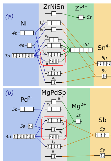
Figure 5. Schematic MO diagram for ZrNiSn (modified from Zeier et al. 5 ) (a) and MgPdSb (b). Orbital energies are not shown to scale.
