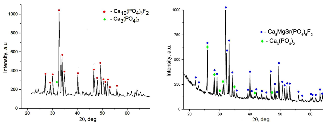
Figure 4. XRD patterns of \text{Ca}_{10}(\text{PO}_4)_6\text{F}_2 (a) and \text{Ca}_8\text{MgSr}(\text{PO}_4)_6\text{F}_2 (b) samples after sintering (1250 °C, 6 h)
