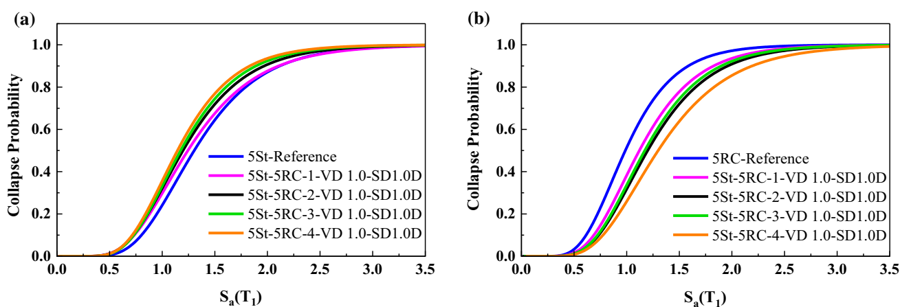
Fig. 21 Seismic fragility curves of a the 5-story SMRF, b the 5-story RC MRF in pounding condition including NPL record subset for SD of 1.0D
