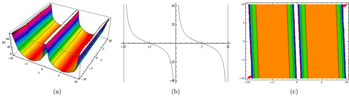
Fig. 18. The graphical presentation of U_2(\xi) given by Eq. (33).
