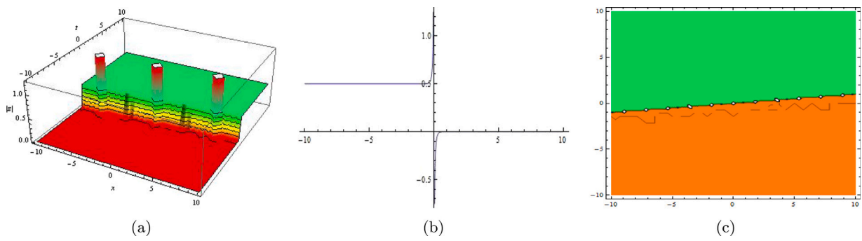
Fig. 7. The graphical presentation of U_2(\xi) given by Eq. (20).
