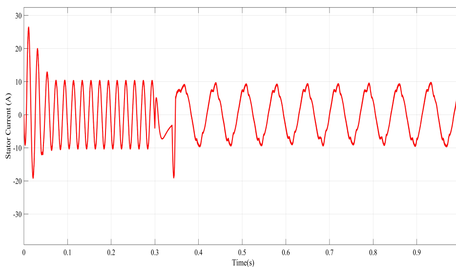
Figure 11. Stator current response to varying load torque.
