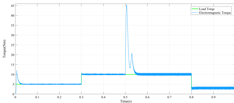
Figure 5. Electromagnetic torque response to step change in speed and load torque.
