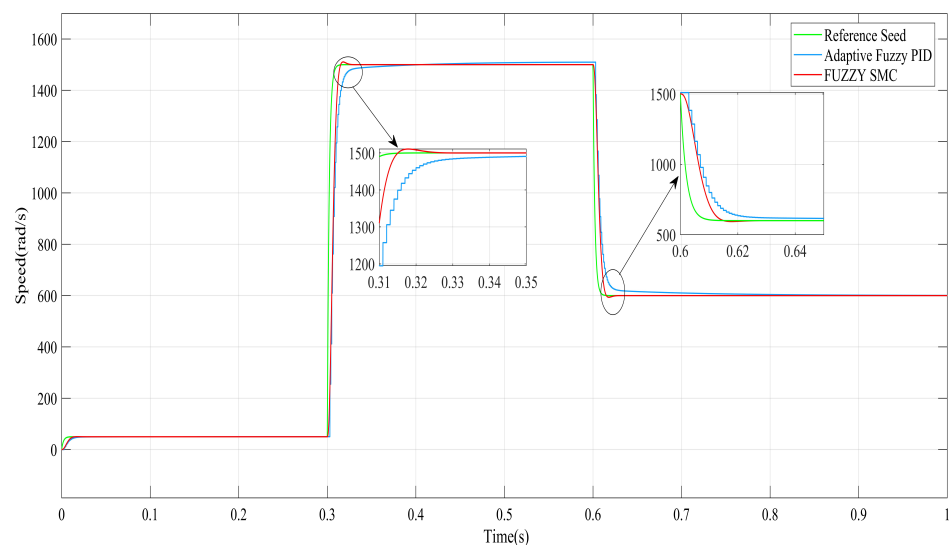
Figure 16. Measured speed to step change with controllers.
