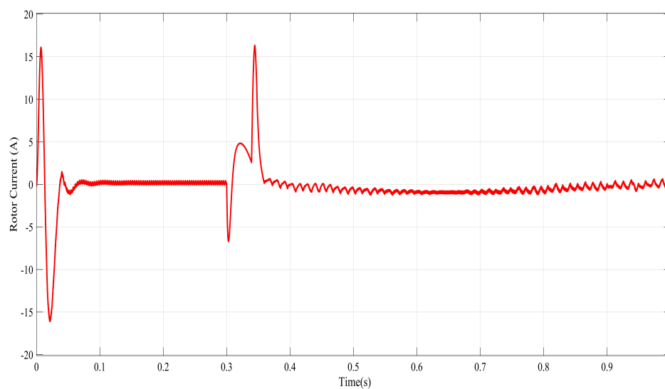
Figure 10. Rotor current response to varying load torque.
