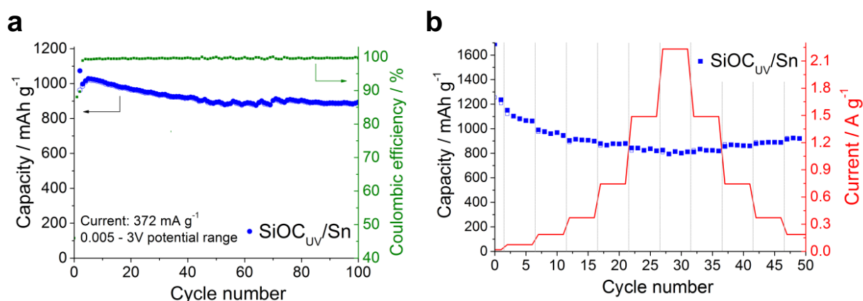
Figure 8.9. a) Cycling stability and b) rate capability performance of SiOC/Sn sample in 5 mV- 3 V potential range. 293
