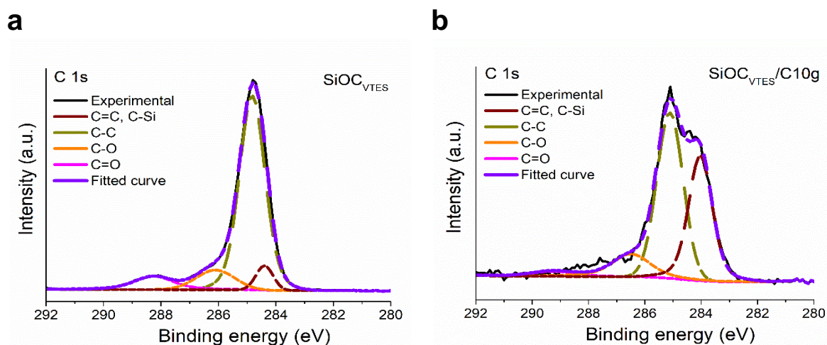
Figure 7.9. XPS C1s spectra of a) SiOC VTES , b) SiOC VTES /C10g samples. 257
