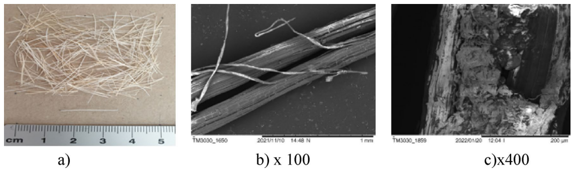
Figure 8. SEM of sisal fibre [Fot.M.Kurpińska].
