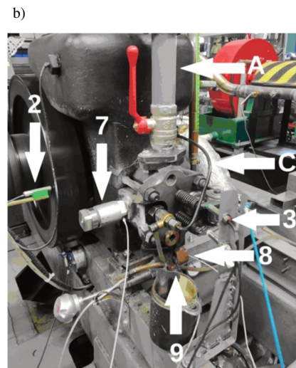
Fig. 6. a) Diagram of the laboratory test stand with the sensor mounting locations marked: 1 – Farymann D10 engine, 2 – engine rotational speed and TDC sensor, 3 – exhaust valve opening sensor, 4 – A/C converter, 5 – recorder, 6 – software, 7 – component to increase the volume of the combustion chamber, 8 – pressure sensor, 9 – water cooled thermocouple, 10 – exhaust gas channel, A – intake air with ball valve on the channel, B – exhaust gas, C – fuel line; b) view of the stand with the location of the sensors highlighted: 2 – engine speed and TDC sensor, 3 – exhaust valve opening sensor, 7 – component to increase the volume of the combustion chamber with a pressure sensor, 8 – pressure sensor, 9 – water cooled thermocouple, A – intake air with ball valve on the channel, C – fuel line
