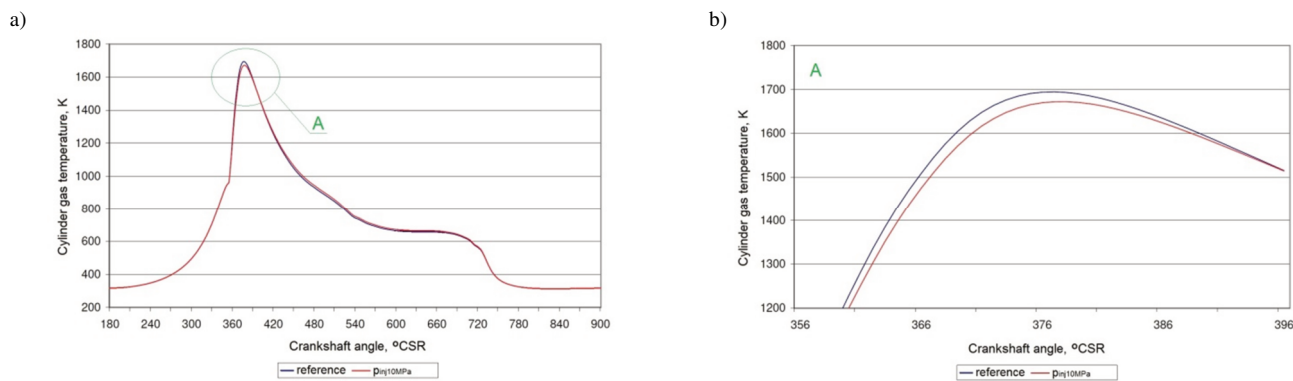
Fig. 2. Courses of changes in the temperature of the working gas in the cylinder T_{cyl} as a function of the angle of rotation of the crankshaft, for the whole working cycle of the engine (a) and for the range of occurrence of the maximum value of the temperature in the cylinder (b), achieved as a result of numerical simulation of the working process of the engine in the program DIESEL-RK under the conditions of introduced changes in the opening pressure of the injector p_{inj}
