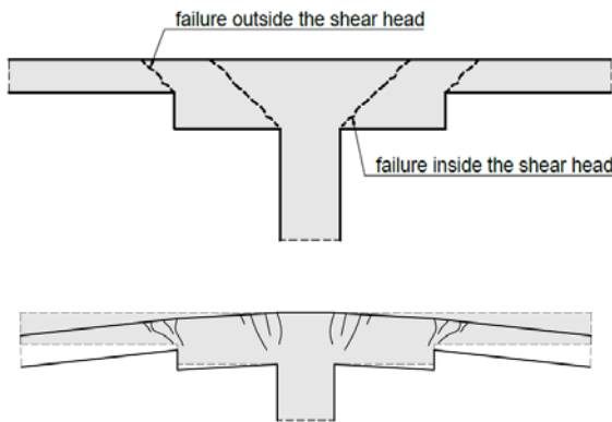
Fig. 1. Column topped with a drop panel: a) potential failure regions; b) drop panel as flexible slab support.
