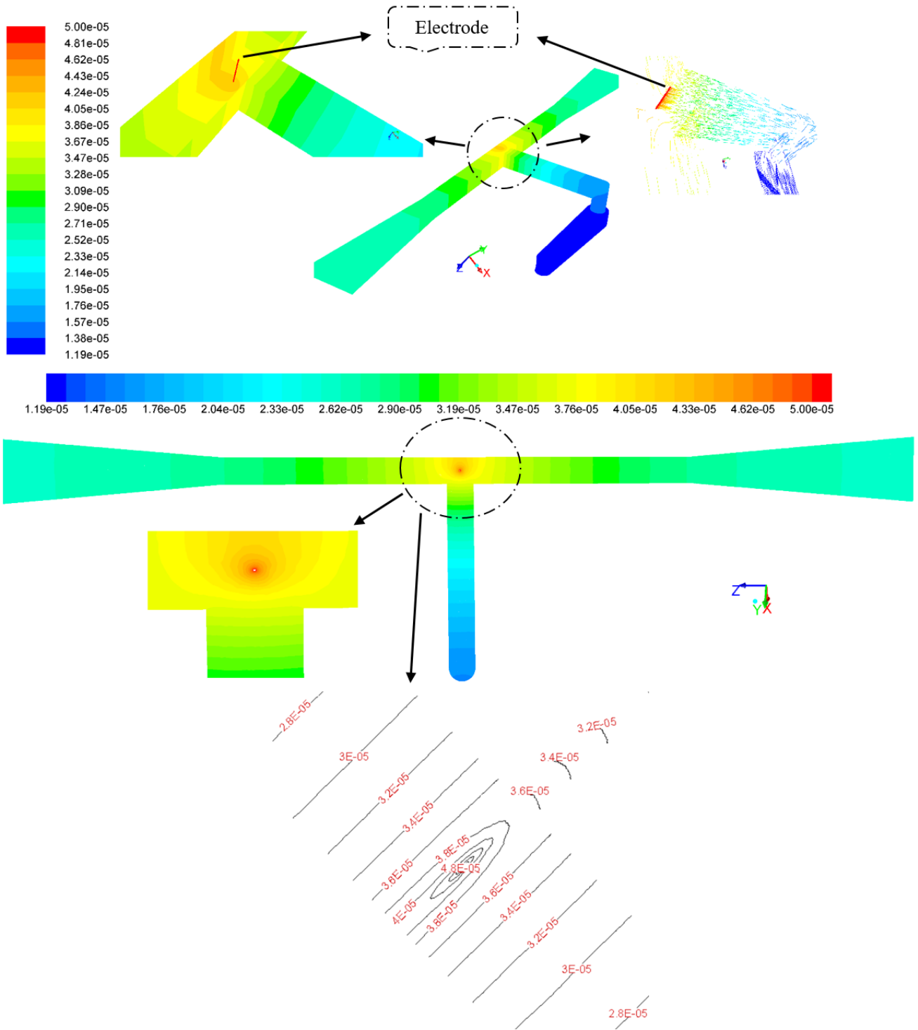
Fig 13. Electric charge contour at voltage 30 KV
