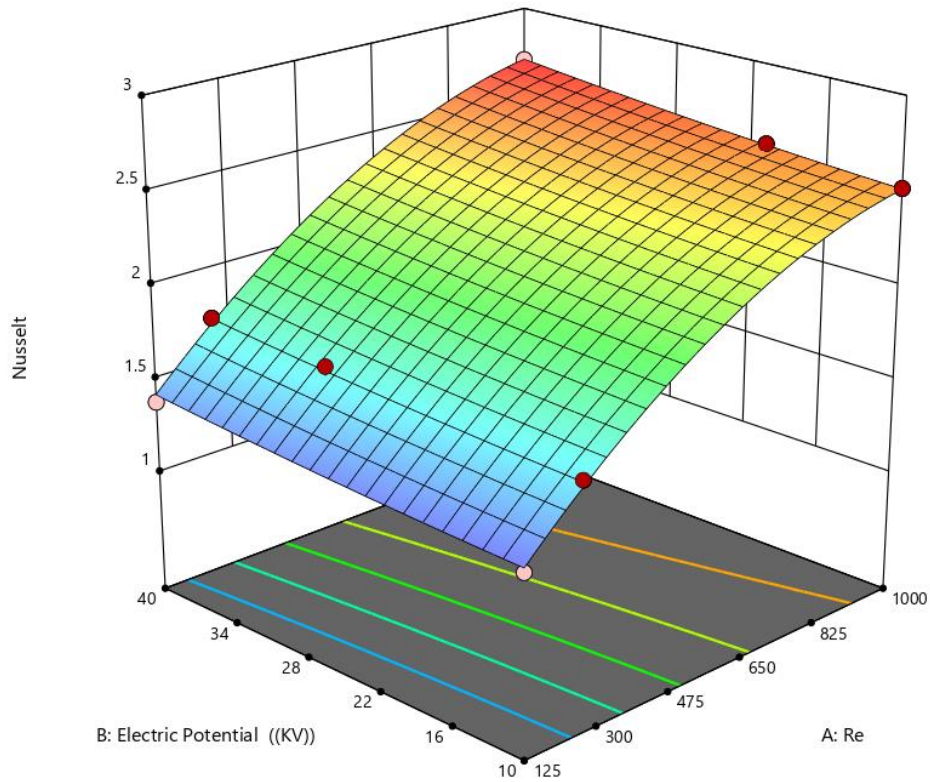
Fig 18. Effects of Reynolds number and applied voltages on local Nusselt number at face1 when \phi_{AL2O3} = \phi_{CuO} = 4\%
