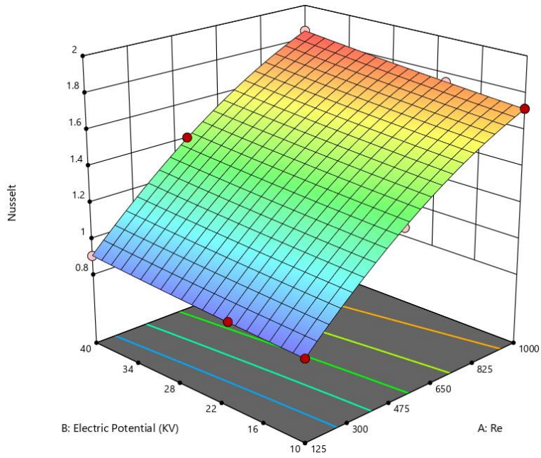
Fig 19. Effects of Reynolds number and applied voltages on local Nusselt number at face2 when \phi_{AL2O3} = \phi_{CuO}
