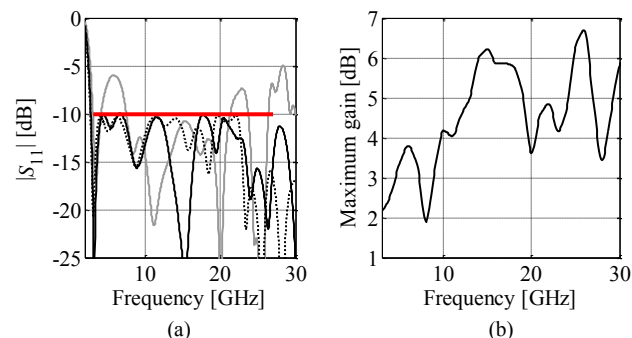
Fig. 2. Characteristics of the proposed antenna: (a) reflection at x^{(0)} (gray), x^* (dotted), and x^* (solid black) designs, and (b) maximum gain at x^* .
