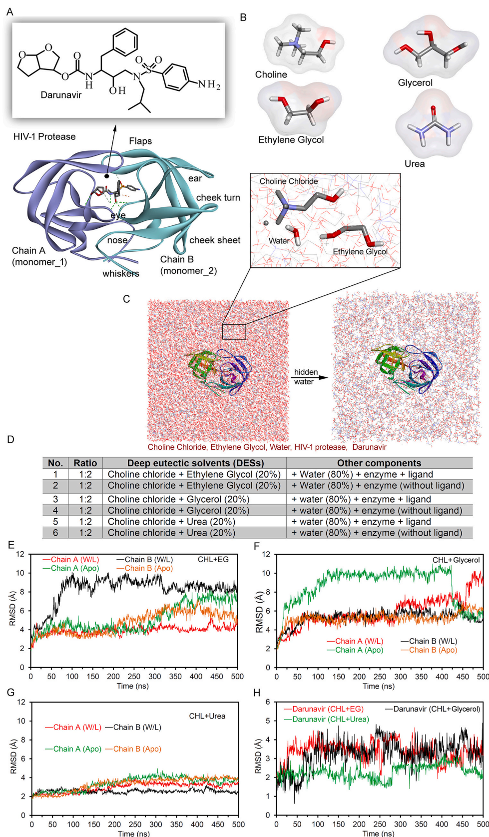
Fig. 1. Components building up systems for protease with different organic solvents. (A) The protease (pdb id.: 4ll3 [27]) enzyme with the Darunavir (Chain A, monomer_1; and Chain B, monomer_2). (B) Structures of different organic solvents: choline chloride (CHL), ethylene glycol (EG), glycerol, and urea with their charge distribution represented as surface. (C) Molecular dynamics simulation (MDS) in periodic boundary conditions (PBC) for the system containing the following components: choline chloride, ethylene glycol, water, protease, and Darunavir. The top right panel represents MDS in PBC with hidden water molecules. (D) Parameterization of the simulated systems containing the protease enzyme and presence/absence of the Darunavir compound consisting of different organic solvents. For each constructed modelled system, 500 ns MD simulations were performed. (E) The RMSDs (root-mean-square deviation; excluding hydrogen atoms) of protease in presence or absence of Darunavir in the system containing choline chloride and ethylene glycol. (F) The protease enzyme in the presence or absence of Darunavir ligand in the system consists of CHL and glycerol. (G) The systems containing choline chloride and urea with HIV-1 protease (with or without ligand). (H) RMSDs for the Darunavir molecule complexed with the protease enzyme in different solvents. (For interpretation of the references to colour in this figure legend, the reader is referred to the web version of this article.)
