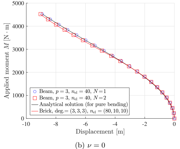
Fig. 10: Lateral contact of a straight beam: Comparison of the X -displacement at the point A (marked in Fig. 9a) for two values of Poisson's ratio: \nu = 0.25 and \nu = 0 . No contact condition is imposed.
