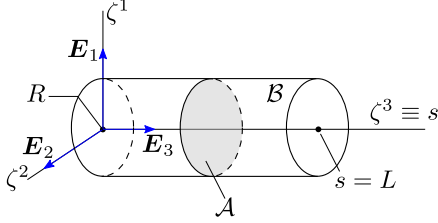
Fig. 2: An example of the reference domain \mathcal{B} in the case of circular cross-section with radius R .
