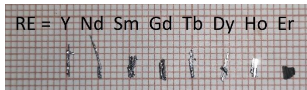
Fig. 3. Single crystals of \text{RE}_3\text{Ni}_5\text{Al}_{19} compounds grown with self-flux method.
