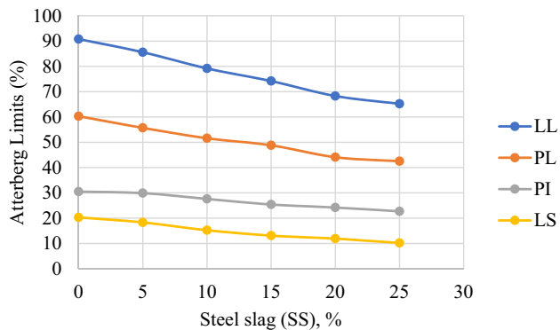
Fig. 5 Variation of Atterberg limit on steel slag (SS)
