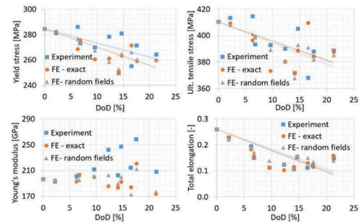
Figure 4. Numerical modelling and experiment in mechanical properties of 6 mm specimens (Woloszyk and Garbatov 2022).
