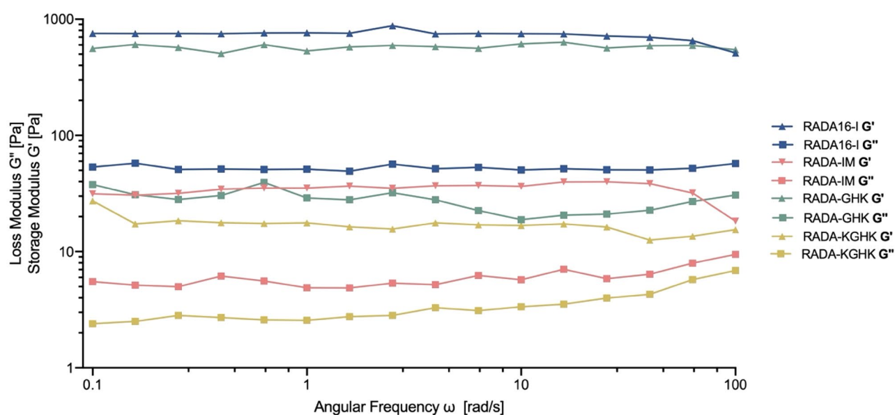
Figure 9. Mechanical characterization of hybrid peptides by dynamic frequency sweep test, at 1% concentration, \gamma = 1\% , 37\text{ }^{\circ}\text{C} .
