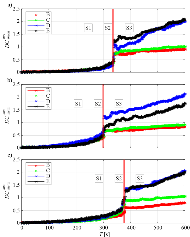
Fig. 8. Decorrelation diagrams of moving reference trace for mean values of k = 1 : n : a) beam #1, b) beam #2, c) beam #3
