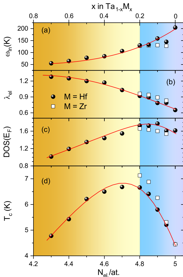
FIG. 11. Valence electron count ( N_{\text{el}}/\text{at.} ) dependence of (a) the logarithmically averaged phonon frequency ( \omega_{\text{ph}} ), (b) electron-phonon coupling constant, (c) electron density of states at the Fermi energy [ \text{DOS}(E_F) ], and (d) superconducting critical temperature ( T_c ). The red solid lines are guide lines. The top axis shows the Hf or Zr concentration ( x ) in \text{Ta}_{1-x}\text{M}_x .
