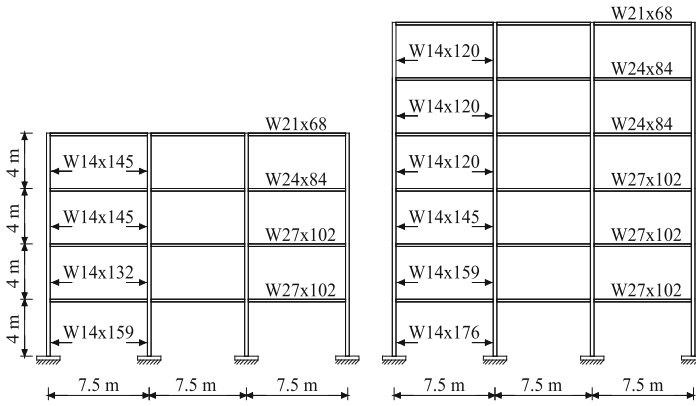
Fig. 1. Structural details of the 4-, and 6-Story frames.
