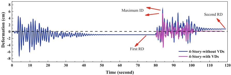
Fig. 3. Comparing the deformation results of the 4-Story frame in the seismic mainshock-aftershock analysis with and without VDs.
