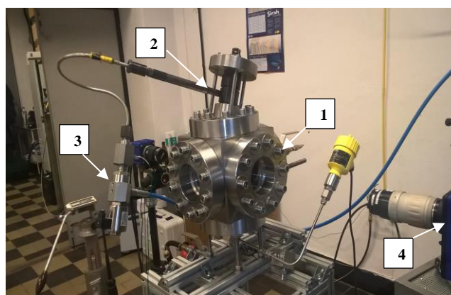
Fig. 1. Experimental laboratory set-up: 1 – constant volume chamber, 2 – marine diesel engine injector, 3 – Kistler 4067E pressure sensor, 4 – high-speed camera
