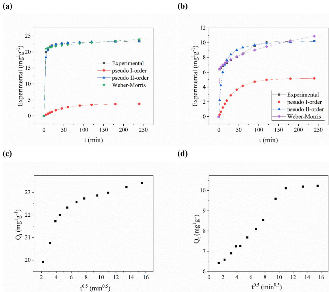
Fig. 3 Kinetic graphic of the adsorption of a RhB and b Cr(VI) made with corn cobs activated carbon. Weber-Morris kinetic plots of c Rhodamine B adsorption and d chromium(VI) adsorption
