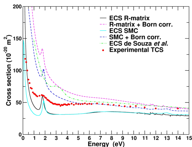
Figure 3. Cross sections for electron scattering on HCOOCH 3 in the low-energy range: experimental grand -total cross section (TCS), elastic cross sections (ECS) obtained with SMC and R-matrix methods with and without Born correction, and ECS obtained with MCOP calculations by de Souza et al. 17
