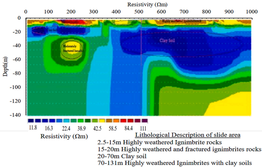
Fig. 7. Muje Ber site electrical profiling 2.
