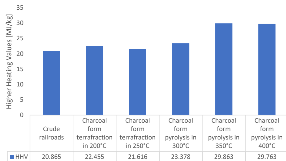
Figure 10. The higher heating value of the raw material (20 °C) and the chars obtained with different final temperatures.
