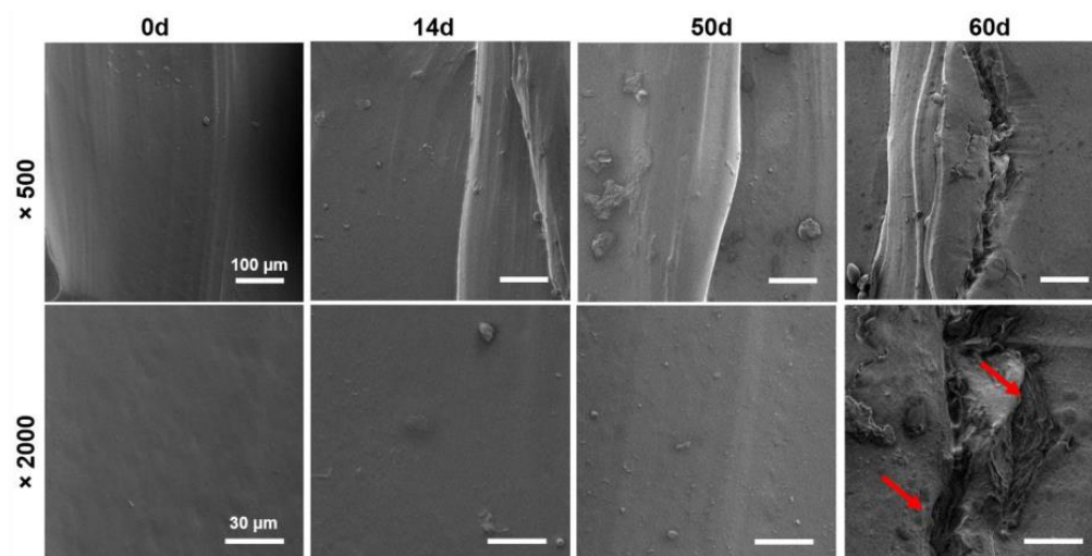
Figure S4 SEM images of the FF_P during a laboratory-scale composting test. The red arrows indicate cracks in the surface of the sample formed during the composting process.
