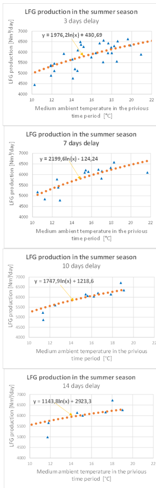
Fig. 9. LFG production model verification process for several days of the observation process
