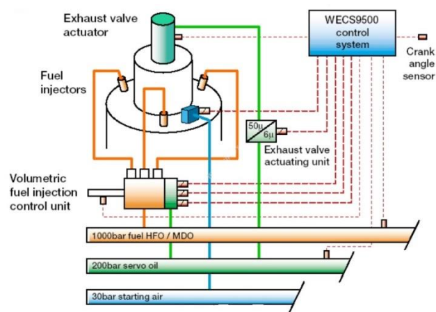
Fig. 5. Wärtsilä RT flex fuel supply system [6]
