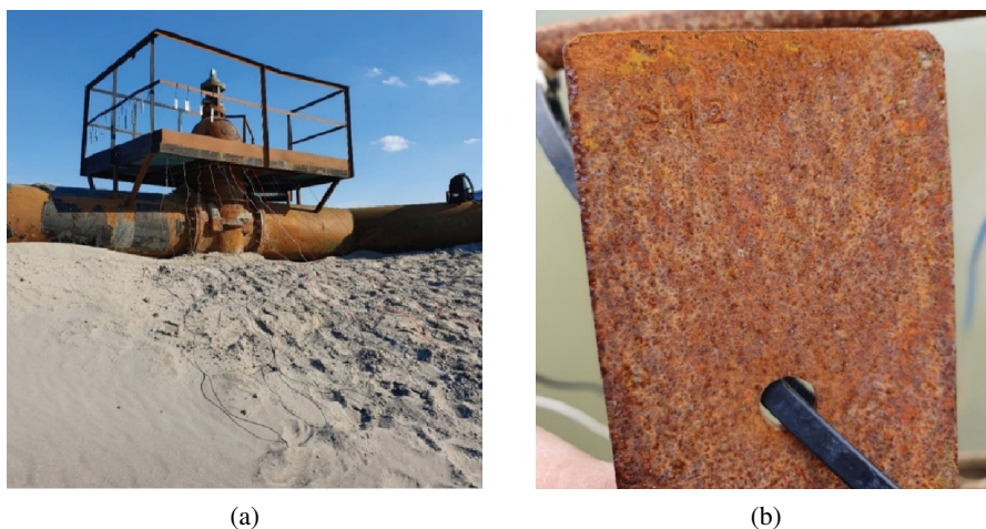
Fig. 4. Exposure of corrosion coupons: a) corrosion coupons, various types of steel – exposure in air and in post-flotation tailings – OUOW \dot{Z} elazny Most, Western Dam, b) corrosion coupon made of S235JR steel after four months of exposure to air – filtration water reservoir, Tarnówek pumping station
