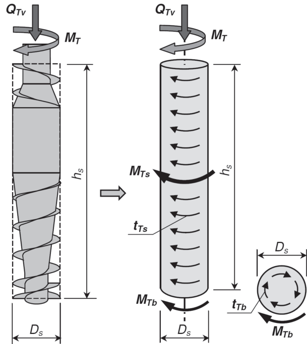
Figure 5: Auger and its simplified schematic representation (right) in the form of a cylinder (Krasieński, 2014).
