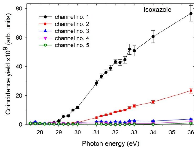
Figure 3. The coincidence yields of two-body dissociation channels following double photoionization of isoxazole in the 27.5-36 eV photon energy range (the assignments of the channels are given in Table 1).
