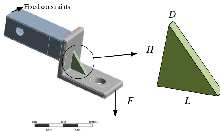
Figure. 13. Support bracket
