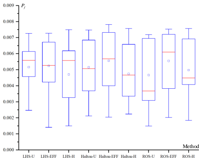
Figure. 28. Boxplot of maximum failure probability for cantilever beam engineering example
