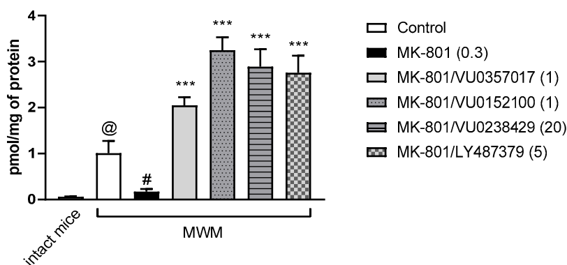
Figure 10. The effect of the Morris Water Maze (MWM) procedure on cGMP synthesis, and the effect of the investigated compounds in the frontal cortex (A) and hippocampus (B) of MWM-trained mice. The values are expressed as the means \pm SEMs. @ p < 0.001 vs. intact mice, # p < 0.001 vs. MK-801-treated animals, and *** p < 0.0001 vs. the MK-801-treated animals (N = at least 8–10).
