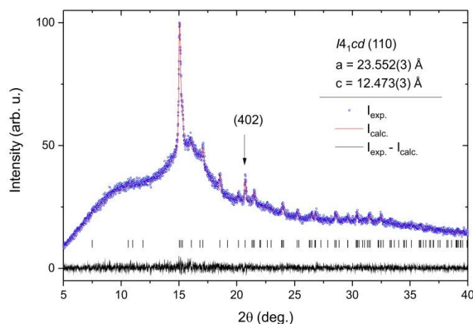
Figure 2. XRPD patterns for compound 1 of the general formula \text{CoM}_2 .
